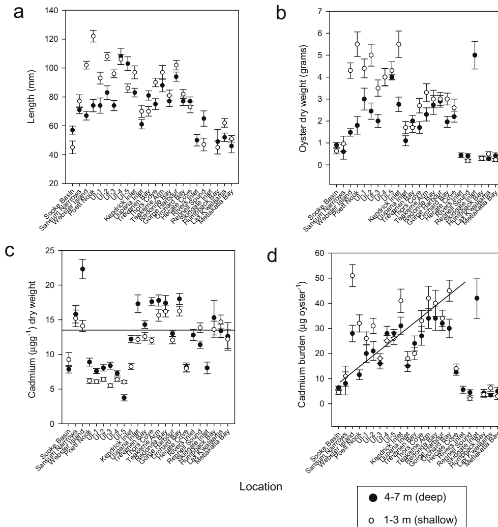
Fig. 3. (a–d). Oyster length, dry weight, cadmium concentration and cadmium burden (mean \pm 1 S.E.) for each location. Sites are plotted in a south to north direction. Reference bar on Fig. 3c is the 13.5 \mu\text{g g}^{-1} dry weight or 2 \mu\text{g g}^{-1} wet weight reference point for rejection of oysters from the Hong Kong market.
